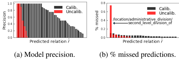
Figure 8: Model performance by relation type. The x-ticks represent relations (labels not shown for brevity).
