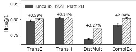
Figure 1: 2D Platt scaling improves \text{hits}@1 for relation prediction on FB15K.
