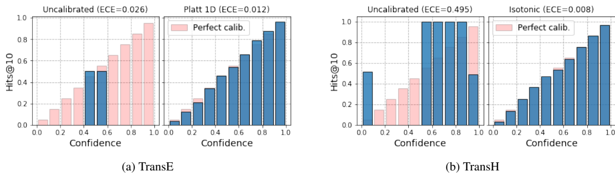
Figure 5: Reliability diagrams for entity prediction on WN18RR.
