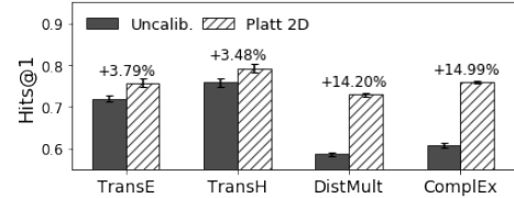
Figure 4: 2D Platt scaling improves hits@1 for relation prediction on WN18RR.
