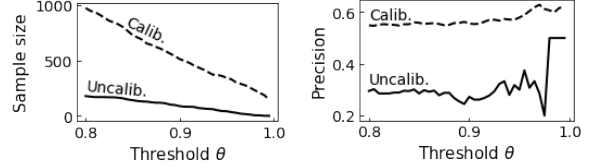
(a) Sample size. (b) Model precision.
