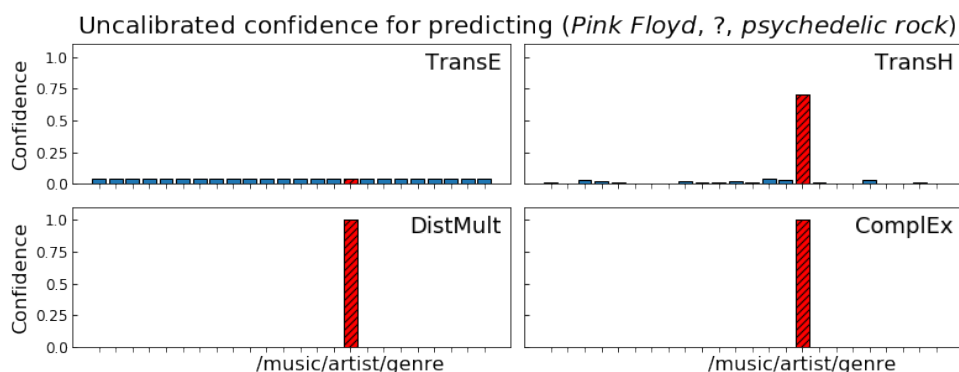
Figure 6: Uncalibrated confidence distributions for predicting the relation in triple (Pink\ Floyd, ?, psychedelic\ rock) in the subset of FB15K containing only relations in the /music domain. The x-ticks represent all relations in the dataset (labels not shown for brevity). The red bar is the ground-truth relation /music/artist/genre .
