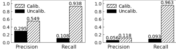
(a) Missing triples (FN). (b) Erroneous triples (FP).
